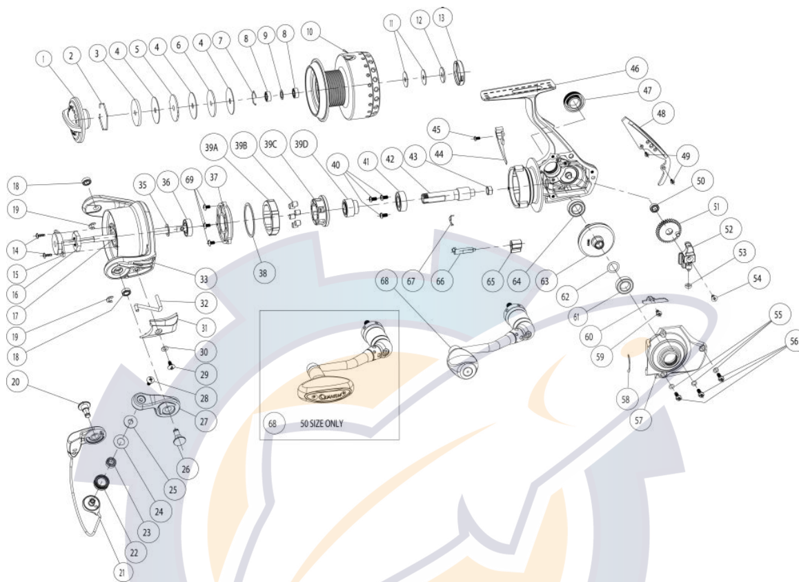
Quantum Energy EI50PTsB Spinning Reel Part List
